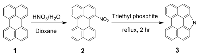
Scheme 1. Synthetic route for pyrroloperylene 3 .
